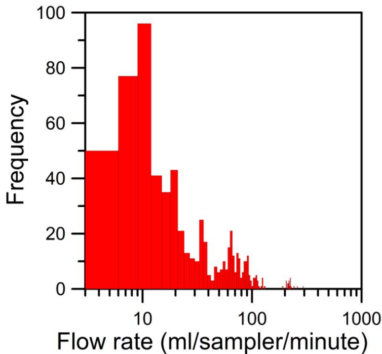
Figure 66: Frequency histogram of seepage measurements made between June 28, 2012, and April 2013 around a spring concentration on the north shore of Deer Lake.
